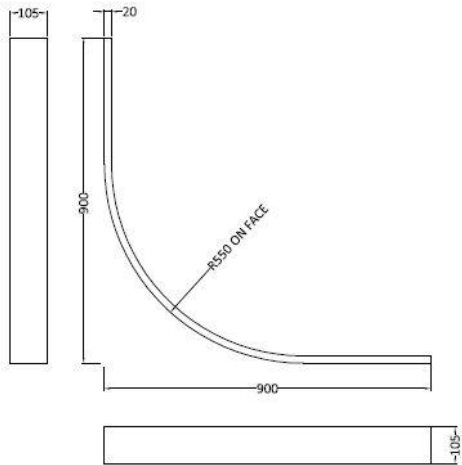
900 x 900 QUADRANT TRAY PANEL
